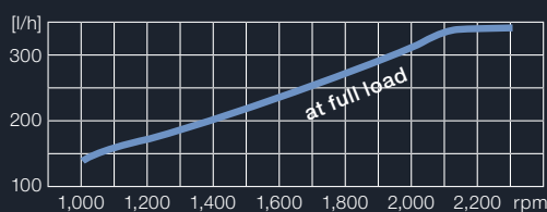
Fuel Consumption V12-1800
